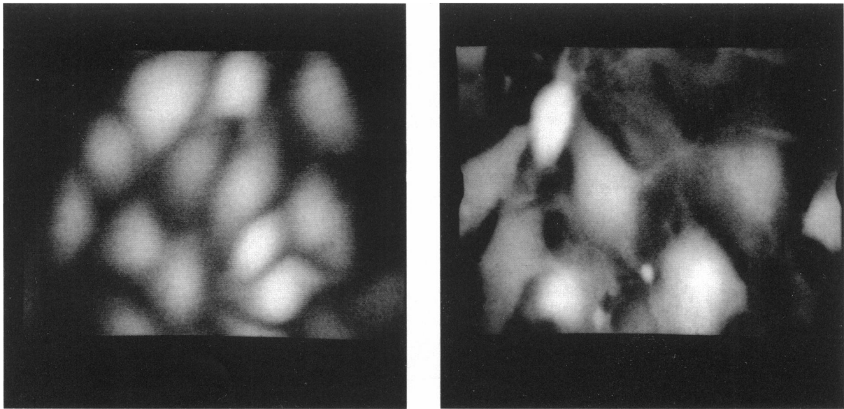
FIGURE 2 Photographs of fibroblasts ( left ) and LLC-PK1 cells ( right ) labeled with SPQ. Cells were perfused with solution 2 at 37°C after SPQ loading and imaged as described in Methods. Background signal measured in the absence of cells was subtracted digitally. Final magnification is 1,250.
