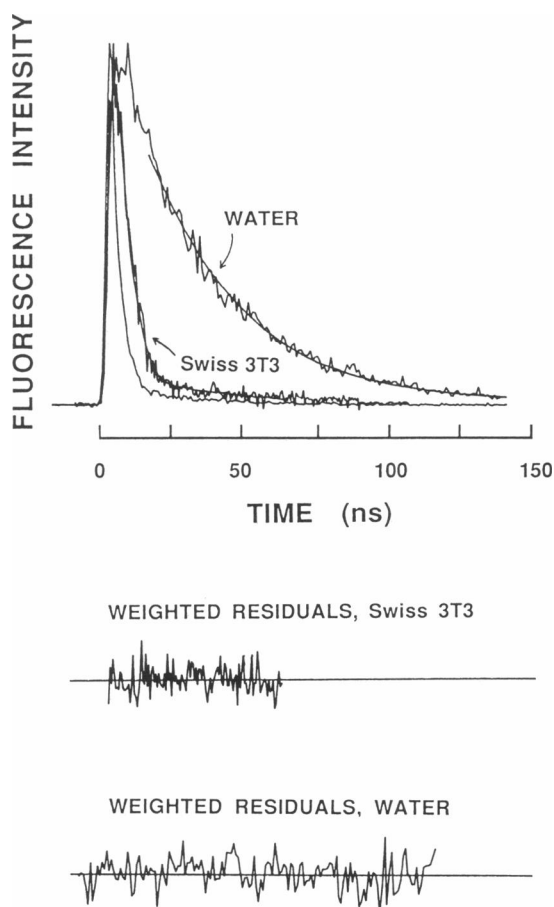
FIGURE 5 Nanosecond SPQ lifetime in a single fibroblast and in free solution. SPQ-loaded fibroblasts were incubated in solution 16 (zero Cl) for 30 min. Free solution SPQ consisted of 100\text{ }\mu\text{M} SPQ in \text{H}_2\text{O} . The decay of fluorescence was measured as described in Methods. Fitted lifetimes and \chi^2 values were 26.0 \pm 0.2\text{ ns} and 1.5 (free solution) and 3.2 \pm 0.2\text{ ns} and 1.1 (fibroblast).
